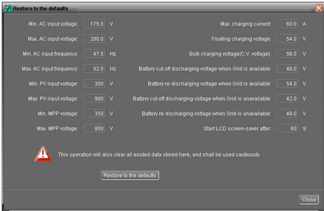
Diagram 4-12B (Off-Grid)
